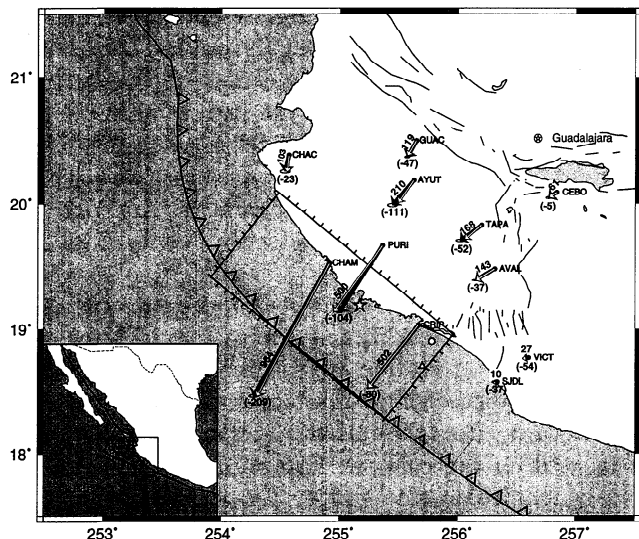
Figure 1. Coseismic displacements for the Oct., 1995, Rivera plate subduction earthquake ( M_w=8.0 ). GPS measurements are shown as solid black vectors, with amount (in millimeters) of horizontal offset written along the vector and vertical offset in parentheses at the vector tip. GPS vectors at stations SJDL and VICT point west. Ellipses represent 2D 95% confidence intervals. Thin white vectors are modeled from slip distribution in Fig. 2. Gridded rectangle is the surface projected model fault plane, and the Harvard and Caltech centroids and the NEIC epicenter are indicated by the star, circle and triangle, respectively. Inset. The Rivera and Cocos plate subduction zones.
