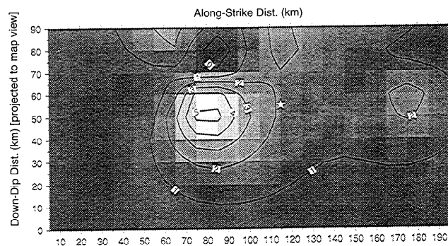
Figure 2. Distribution of slip on the Rivera plate thrust fault. Contours and shading indicate the thrust-slip amplitude (in meters). The model plane has 20 subfaults along-strike and 10 sub-faults down-dip, each 10 km by 10 km. The distribution indicates two distinct slip patches separated by 95 km, in agreement with seismic evidence for a multiple-source event. The star indicates the projected position of the Harvard CMT epicenter.
